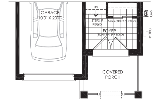
PARTIAL GROUND FLOOR PLAN ELEV. BA
