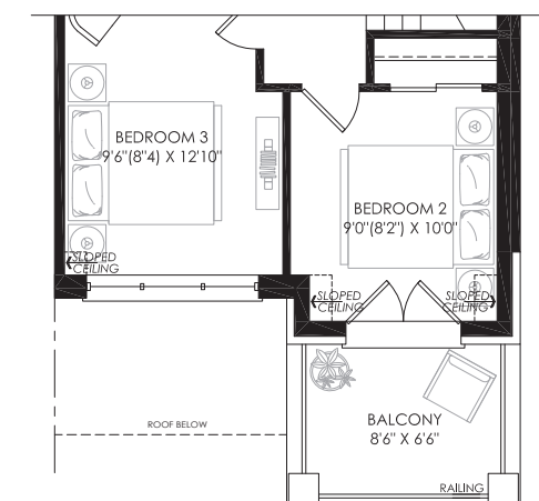
PARTIAL SECOND FLOOR PLAN ELEV. BA
