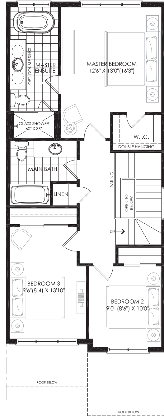
SECOND FLOOR PLAN ELEV. AB
